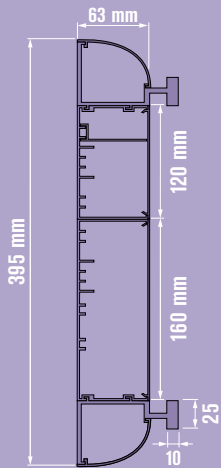
120+160 profiles with high & low rail
