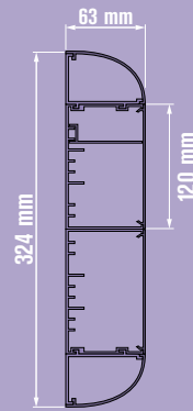
120+120 profiles with high & low finish profiles
