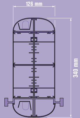
120+120 profiles suspended
