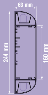
160 profile with general & reading lighting
